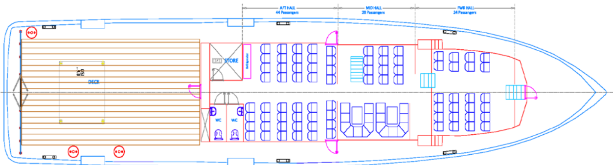
MAIN DECK
