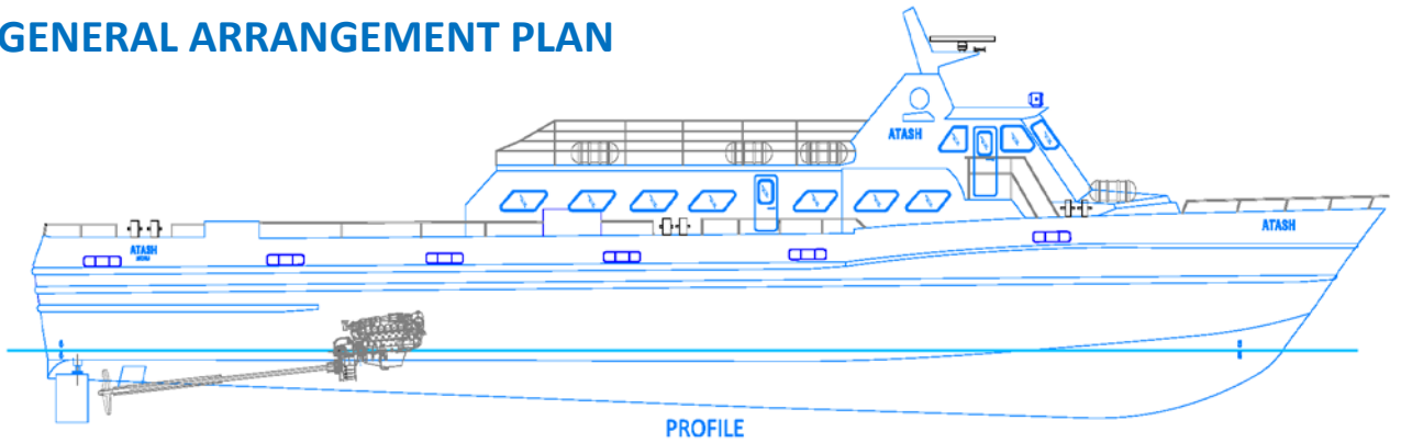
PROFILE
