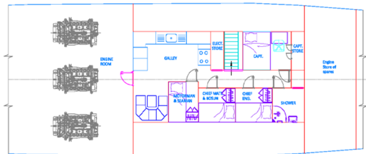
LOWER DECK
